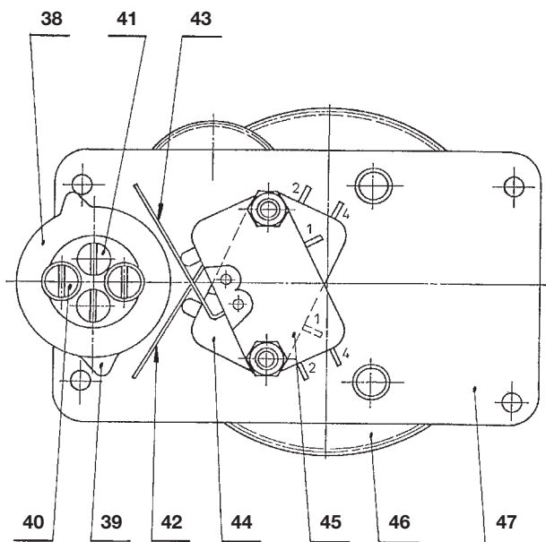
Fig. 4 – Signalling unit
