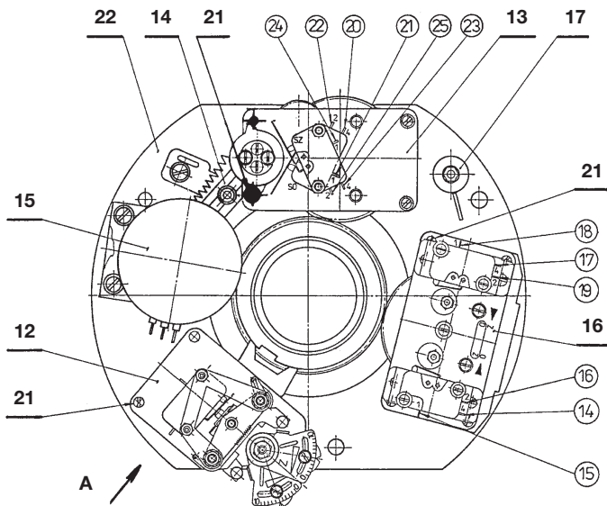
Fig. 2 – Control board – Design with potentiometer 1 x 100 ohm
