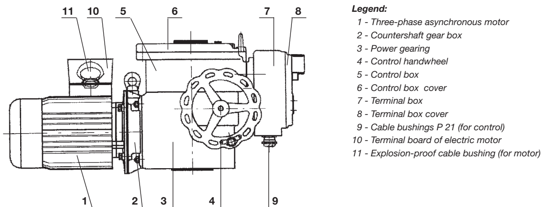
Fig. 1 – Electric actuator configuration
